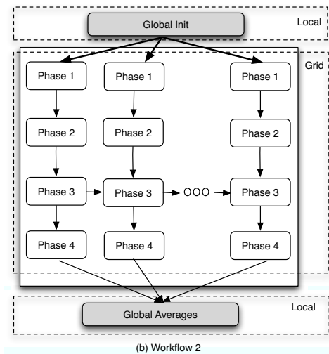
Figure 4. Workflow 2: All parts can be executed on any Grid node including the ones at the submitters site.
